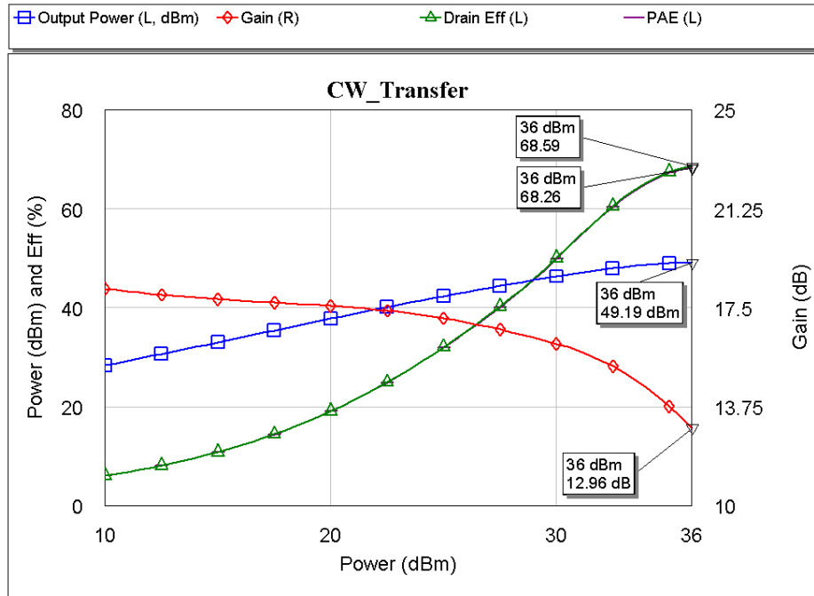
Figure 1. - CGHV60075D Output Power, Gain and Efficiency vs. Input Power at Tcase = 25°C V_{DD} = 50V, I_{DQ} = 125\text{ mA}, \text{Frequency} = 2.7\text{ GHz}
