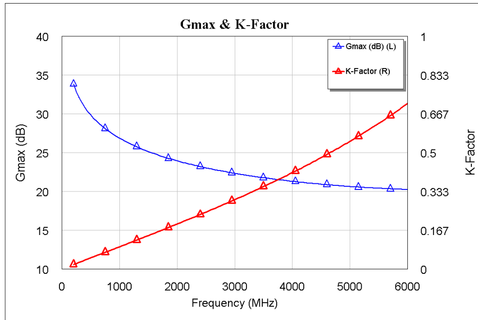
Figure 2. - CGHV60075D GMAX and K Factor vs. Frequency at Tcase = 25°C V_{DD} = 50V, I_{DQ} = 125\text{ mA}
