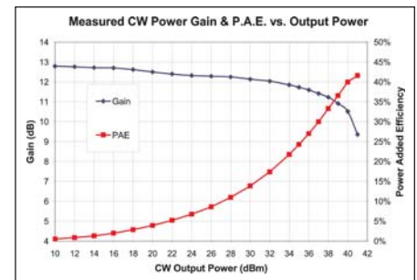
Figure 8 · Measured CW gain and PAE of the CGH35015S demonstration amplifier.
