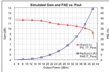
Figure 4 · Simulated gain and efficiency of the amplifier at 3.6 GHz.
