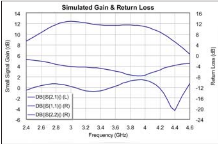
Figure 3 · Simulation of the small signal gain and return loss.
