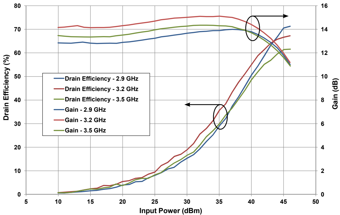
Figure 4. - CGHV35400F Drain Efficiency & Gain vs Input Power
